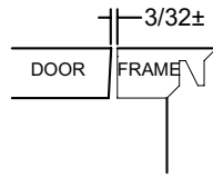
Flush Inset - FI
